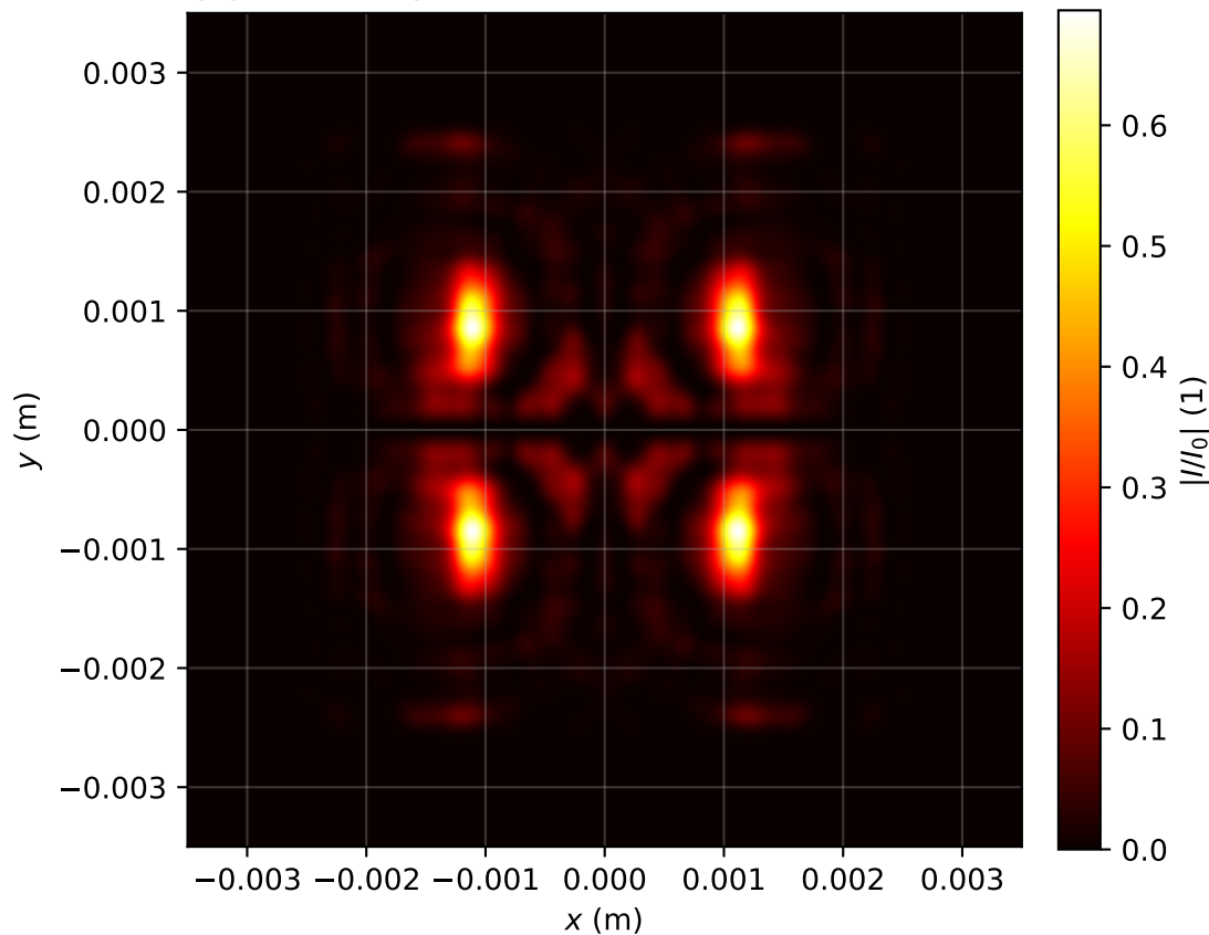
Intensity profile I(x, y, z = 3.025)/I_0 , P_{in}=8.0P_{cr} , artificial time
